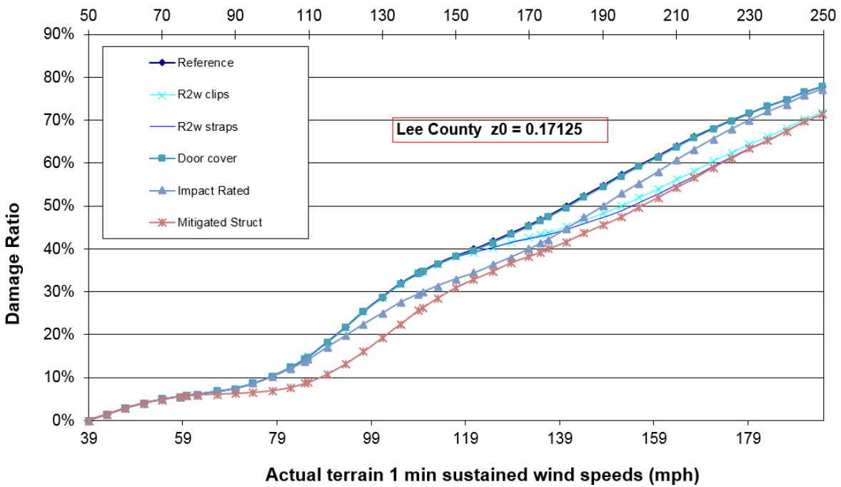
Figure 72. Mitigation measures for masonry homes.
