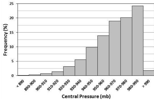
Figure 71. Box Plot and Histogram of Central Pressure vs. R max , Florida and Neighboring States
